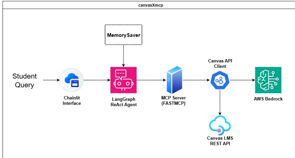
Figure 1: System Architecture
